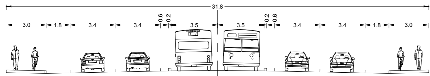
JAPHTA MASEMOLA LINK - NARROW MEDIAN
